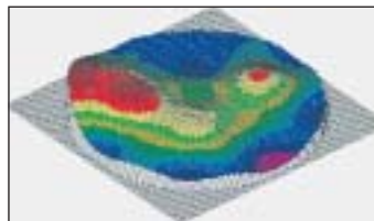
Temperature map of 200 mm wafer showing <1% uniformity at 550°C
